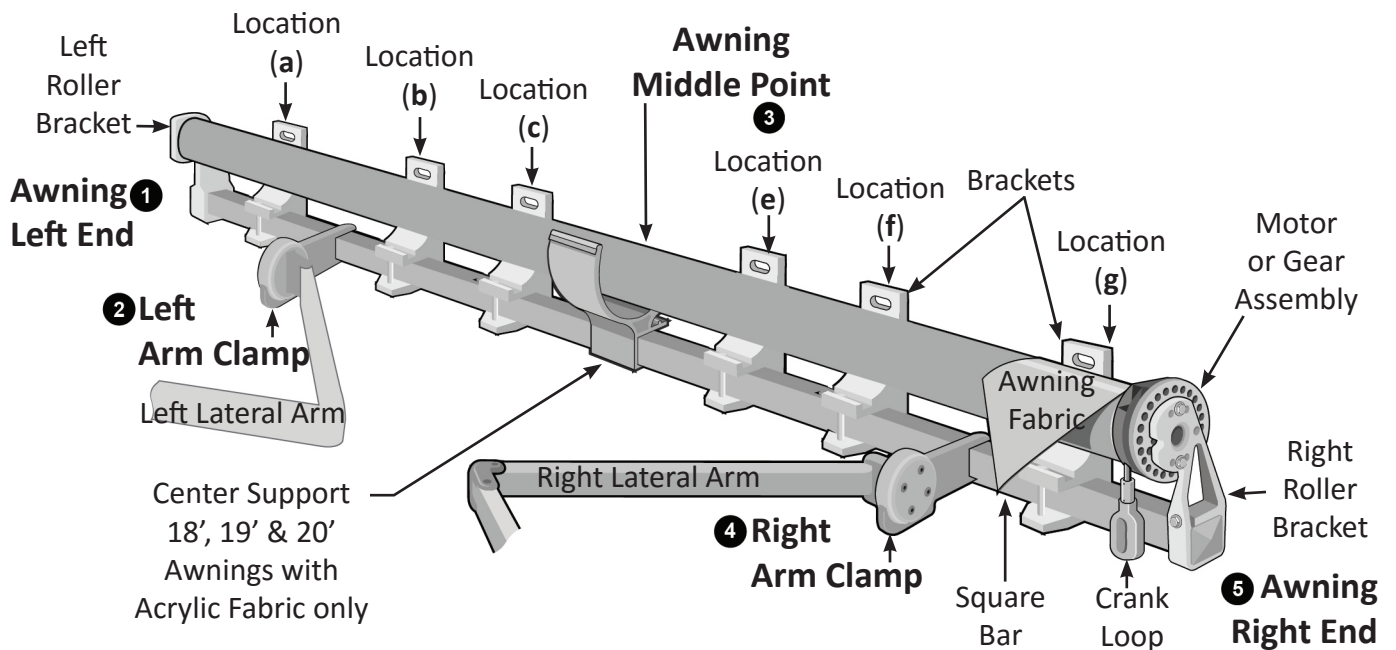
Figure 1d Bracket Locations for 17' - 20' Wide Awnings
