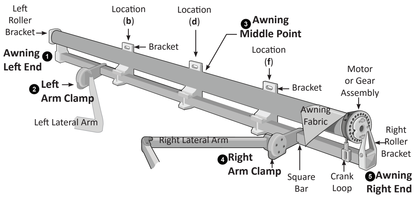
Figure 1b Bracket Locations for 10' - 13' Wide Awnings
