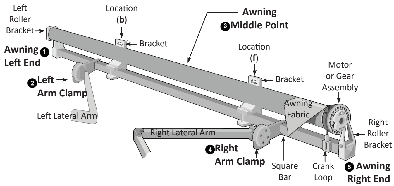
Figure 1a Bracket Locations for 8' Wide Awnings
