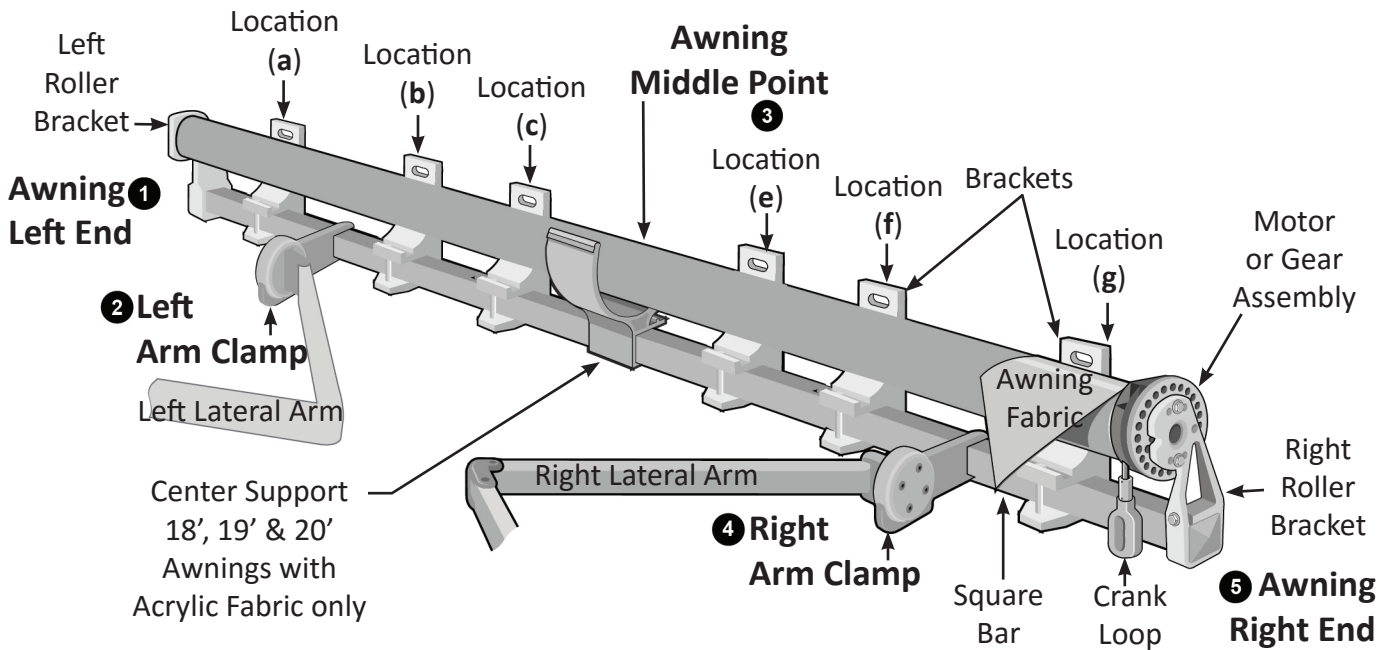
Figure 1d Bracket Locations for 17' - 20' Wide Awnings
